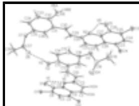
Fig. 1. Structure of 3-[( E )-2-(5,7-dichloro-8-hydroxyquinolin-2-yl)vinyl]-4-hydroxyphenyl acetate showing the atomic numbering scheme. Displacement ellipsoids are drawn at the 50% probability level.
